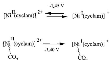
Scheme 2. Reduction of \text{Ni}(\text{cyclam})^{2+} complexes
