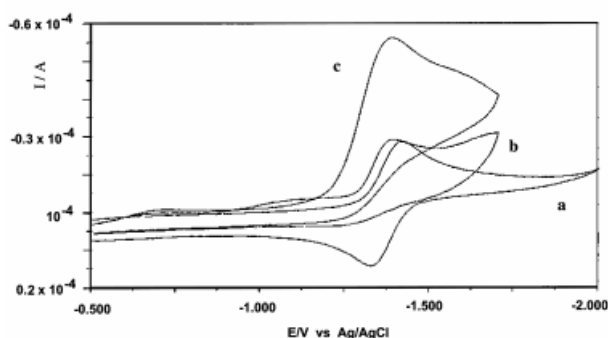
Figure 1. Cyclic voltammetry on a carbon graphite electrode ( v = 100 \text{ mVs}^{-1} ) of a DMF/ n\text{Bu}_4\text{N}^+\text{BF}_4^- solution containing: curve a: [\text{Ni}(\text{cyclam})\text{Br}_2] (2.5 M); curve b: [\text{Ni}(\text{cyclam})\text{Br}_2] (2.5 M) and \text{CO}_2 (saturated solution at 1 atm); curve c: [\text{Ni}(\text{cyclam})\text{Br}_2] (2.5 M) and \text{CO}_2 (saturated solution at 1 atm) + 1a (3 equiv.)
