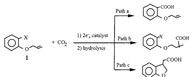
Scheme 1. Possibilities of electrocarboxylation of substrates 1
