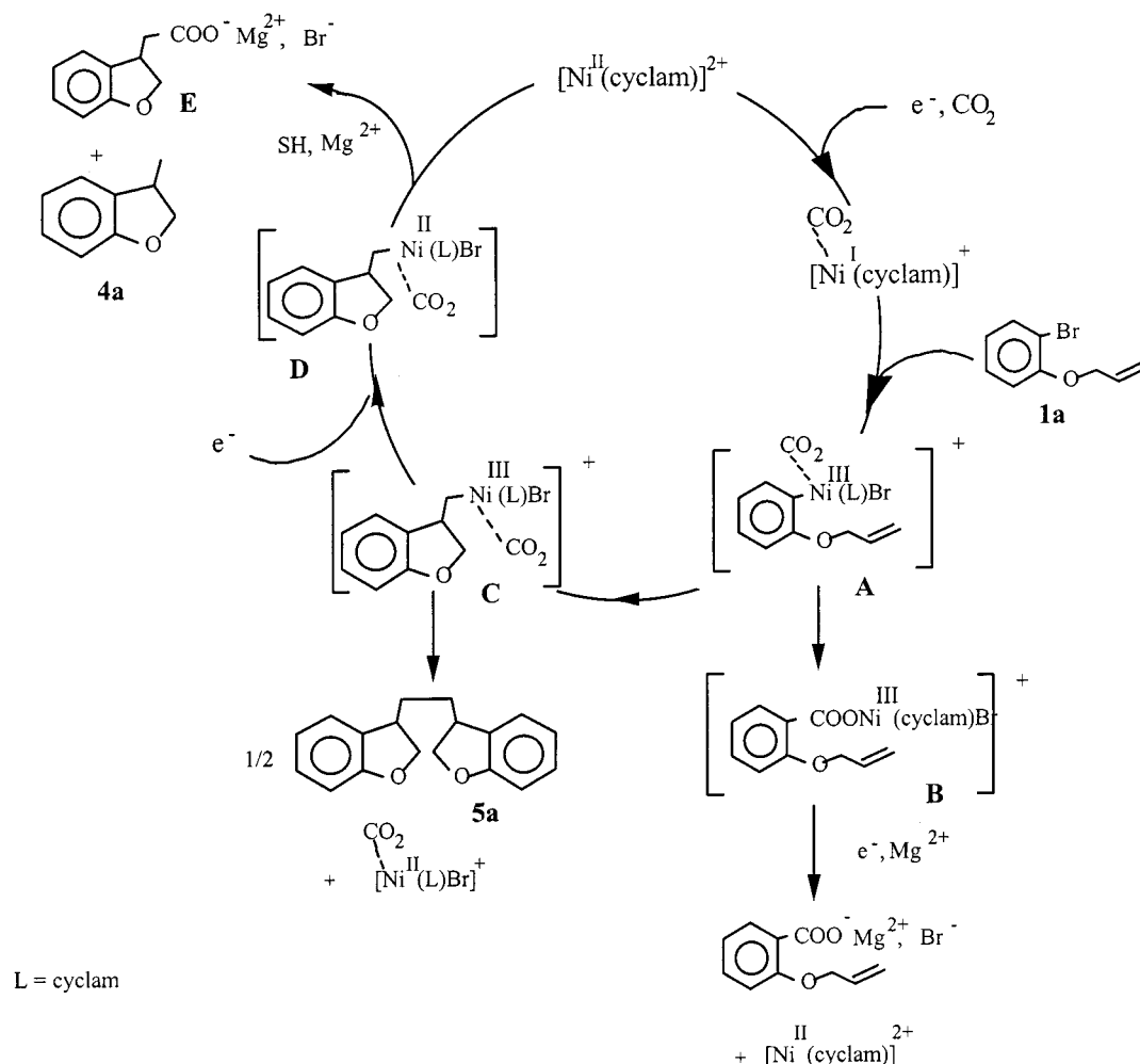
Scheme 3. Proposed catalytic cycle
